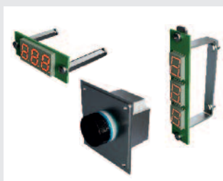
Tap basic (vertikal Display unter dem Ceranglas) Tap basic (horizontal Display unter dem Ceranglas) Tap basic (vertical display under glass) Tap basic (horizontal display under glass)
